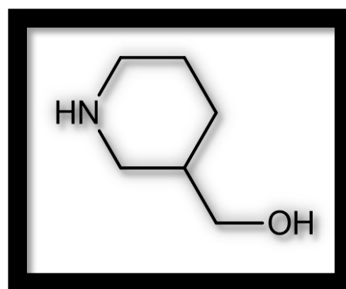
FIGURE 10: The structure of 3-Piperidinemethanol ( 3.79 \times 10^{-3} mol, MW = 115.18)
